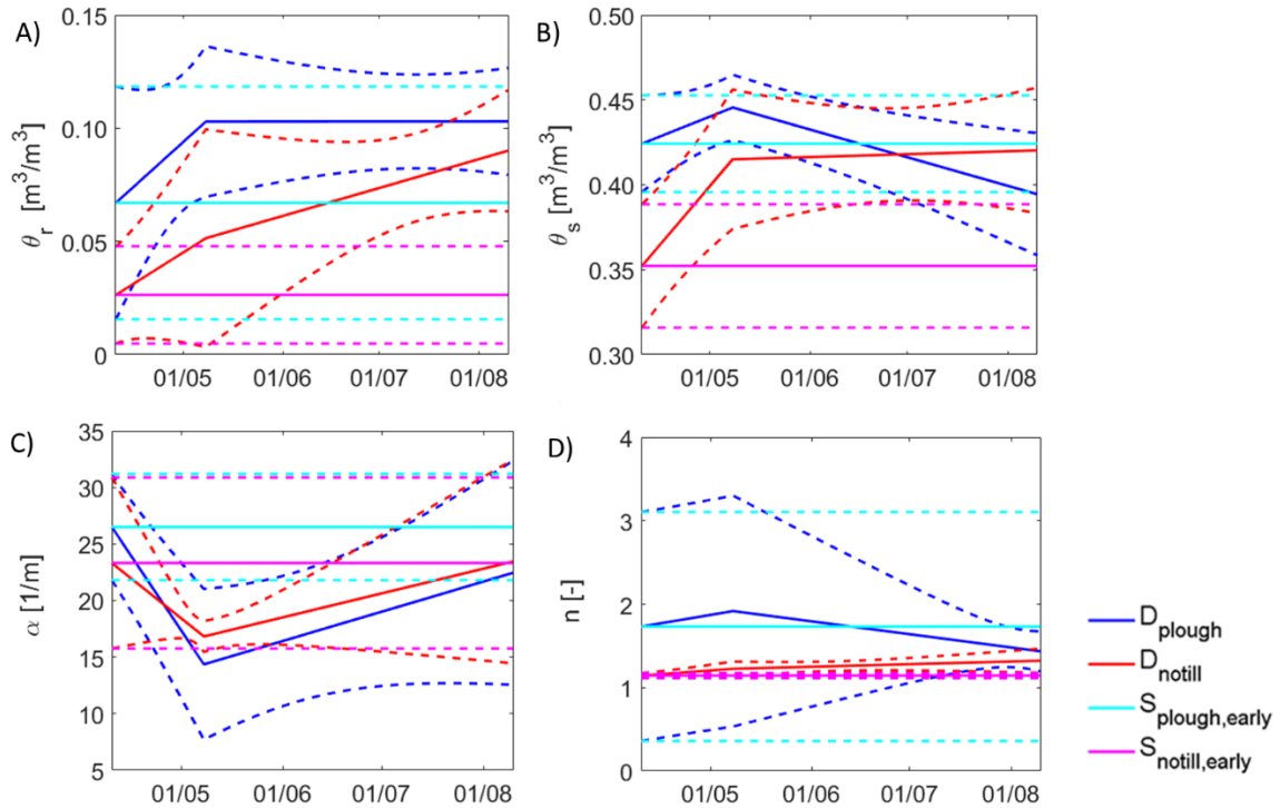
766 Figure 3 Time dynamics implemented in HYDRUS for the pore-size distribution parameters \theta_r , 767 (a), \theta_s (b), \alpha (c), and n (d), for the upper depth ( z_{\text{sample1}} : 0.025\text{m} ) for set of dynamic scenario 768 simulations in the ploughed fields ( D_{\text{plough}} in blue) and in the no-till fields ( D_{\text{notill}} in red), and in 769 the static simulations scenario, where the temporal changes of the soil parameters were 770 omitted. The values of the parameters in the static scenarios were based on the first sampling 771 value in D_{\text{plough}} ( S_{\text{plough}} , in light blue) and in D_{\text{notill}} ( S_{\text{notill}} , in pink). The solid lines represent the 772 average values, the dashed lines represent the ranges (minimum and maximum values) 773 among the 9 replicate samples.
