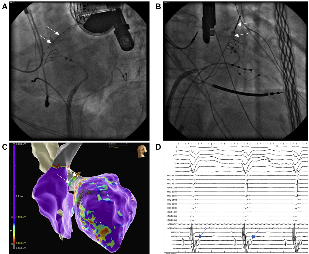
Fluoroscopic images in the (A) left anterior oblique and (B) right anterior oblique projection showing catheter locations during the case. The 2-F octapolar catheter (white arrows in A and B) is positioned in the summit communicating vein. The HD Grid (Abbott Laboratories) is on the adjacent septal surface of the left ventricular cavity. (C) Bipolar voltage map of the left ventricular and left ventricular endocardium in the left anterior oblique projection. Areas of low voltage (<1.5 mV) are seen at the basal-septal left ventricular and periaortic regions, extending toward the apex. The HD Grid is seen within the left ventricular cavity abutting the septum. The 2-F octapolar catheter (white arrows) is also observed in the summit communicating vein extending intraseptally. (D) Fractionated and delayed electrograms (blue arrows) recorded by the 2-F octapolar catheter during sinus rhythm are significantly more prominent than those on the HD Grid situated on the adjacent left ventricular septal surface.
