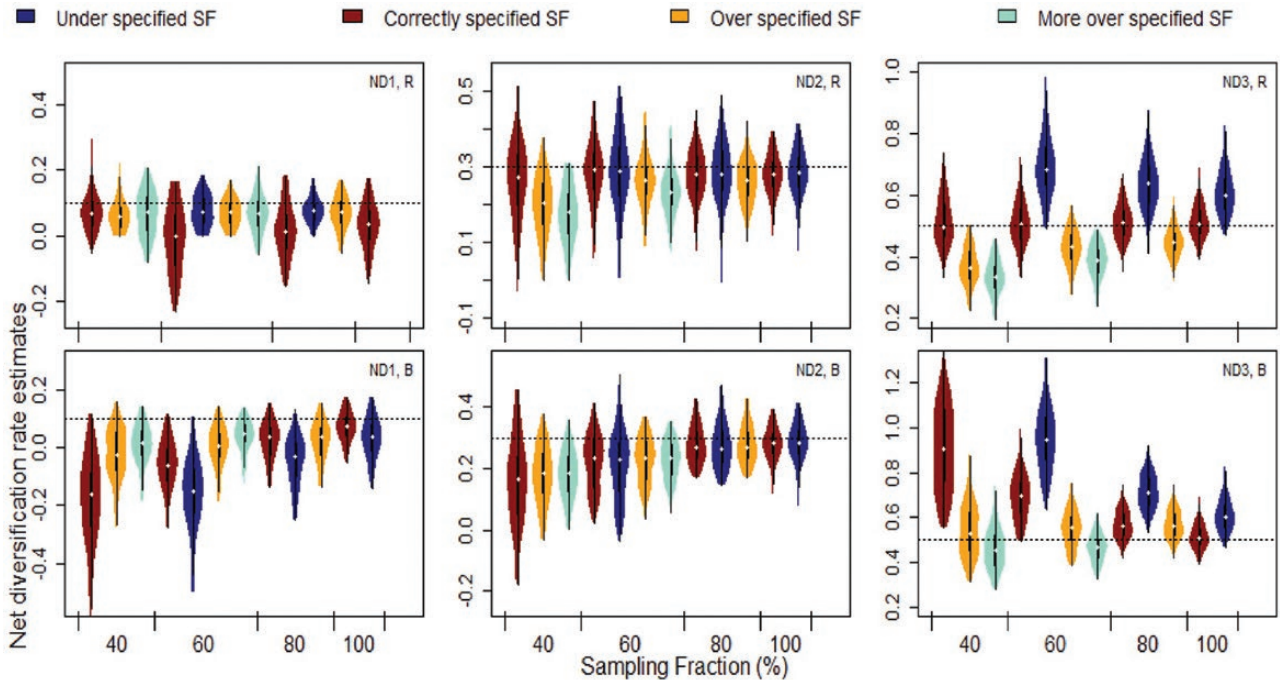
FIGURE 5. Net diversification rate estimates of the medium size ETD generated phylogenetic trees, that were randomly (R; top row) or biased (B; bottom row) trimmed. ND1, ND2 and ND3 indicate the net diversification rate for trait state 1, 2 and 3 respectively. Colors indicate if the SF was correctly specified or mis-specified. The horizontal line indicates the true parameter value. Plots include all generated trees for each set, regardless of whether the generating model was selected as the best model or not.
