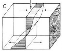
Figure 5. Typical normal stress distribution in a timber beam under bending: yielding may occur on the compressed side, while structural response is linear elastic for tensile stresses.
