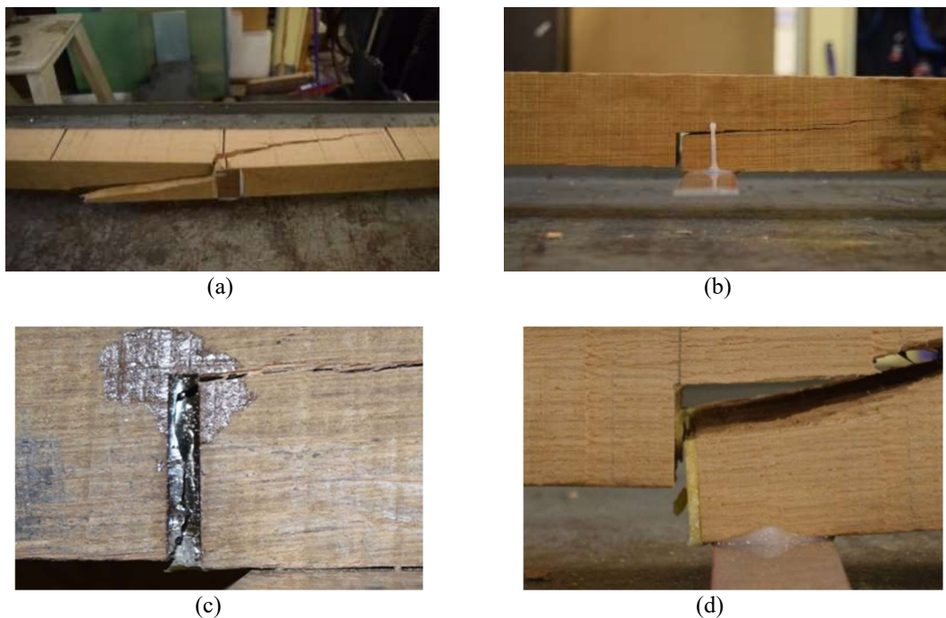
Figure 7. Specimens' failure modes: (a) CT series (control undamaged beams); (b) DUT series (damaged and unrepaired beams); (c) BRT series (damaged and bone glue repaired); (d) RRT series (damaged and rosin repaired).
