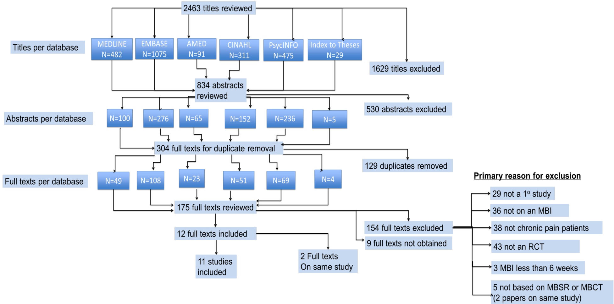
Figure 1: PRISMA flowchart
